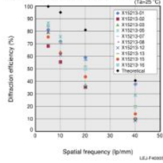
Figure 4: Diffraction efficiency (typical example)
