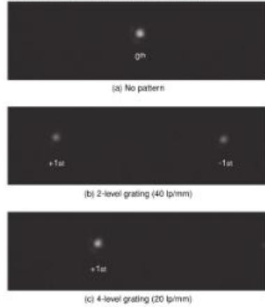
Figure 3: Diffracted spots images (typical example)
