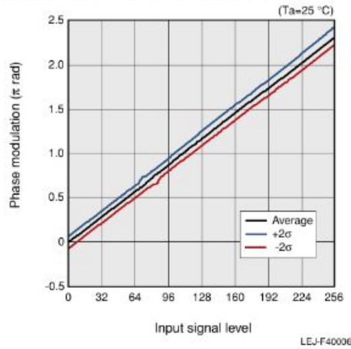
Figure 5: Phase modulation (typical example)
